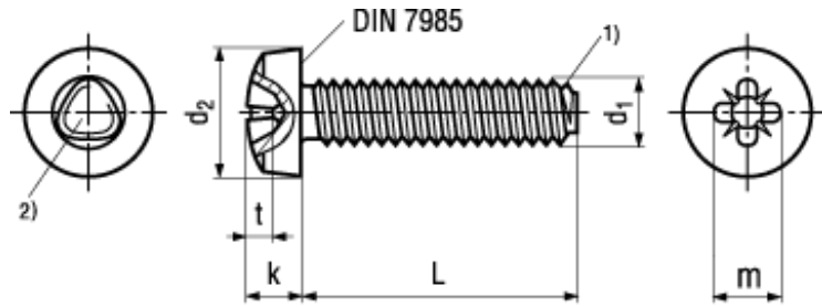
1) Tapered thread end max. 4P 2) Trilobular
